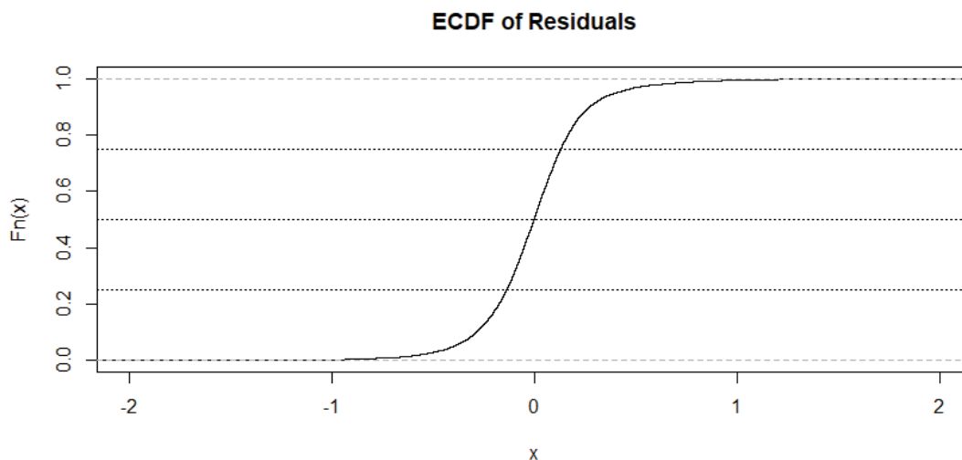
Empirical Cumulative Distribution Function of Residuals
