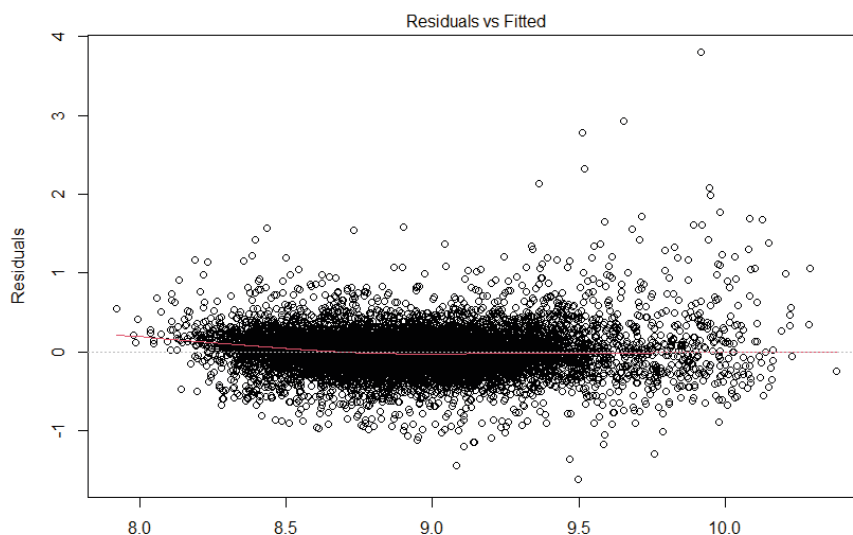
Residual -vs-Fitted Plot
